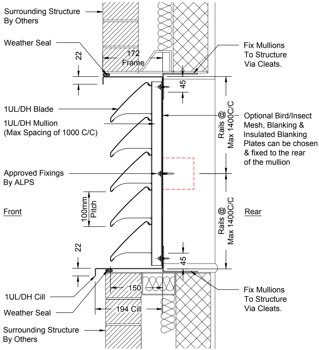
Typical 1ULDH Section
