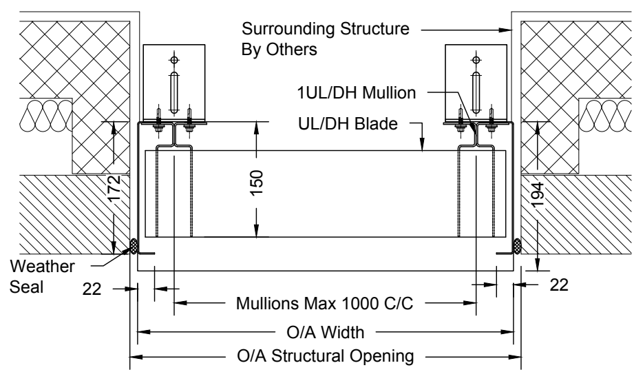
Typical 1ULDH Plan
