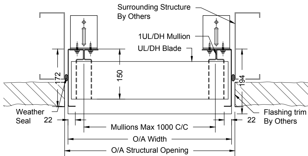
Typical 1ULDH Plan
