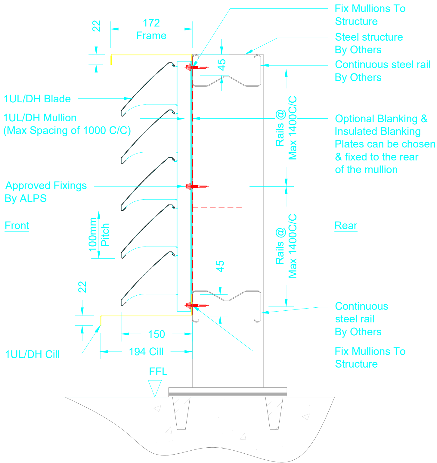
Typical 1ULDH Section
