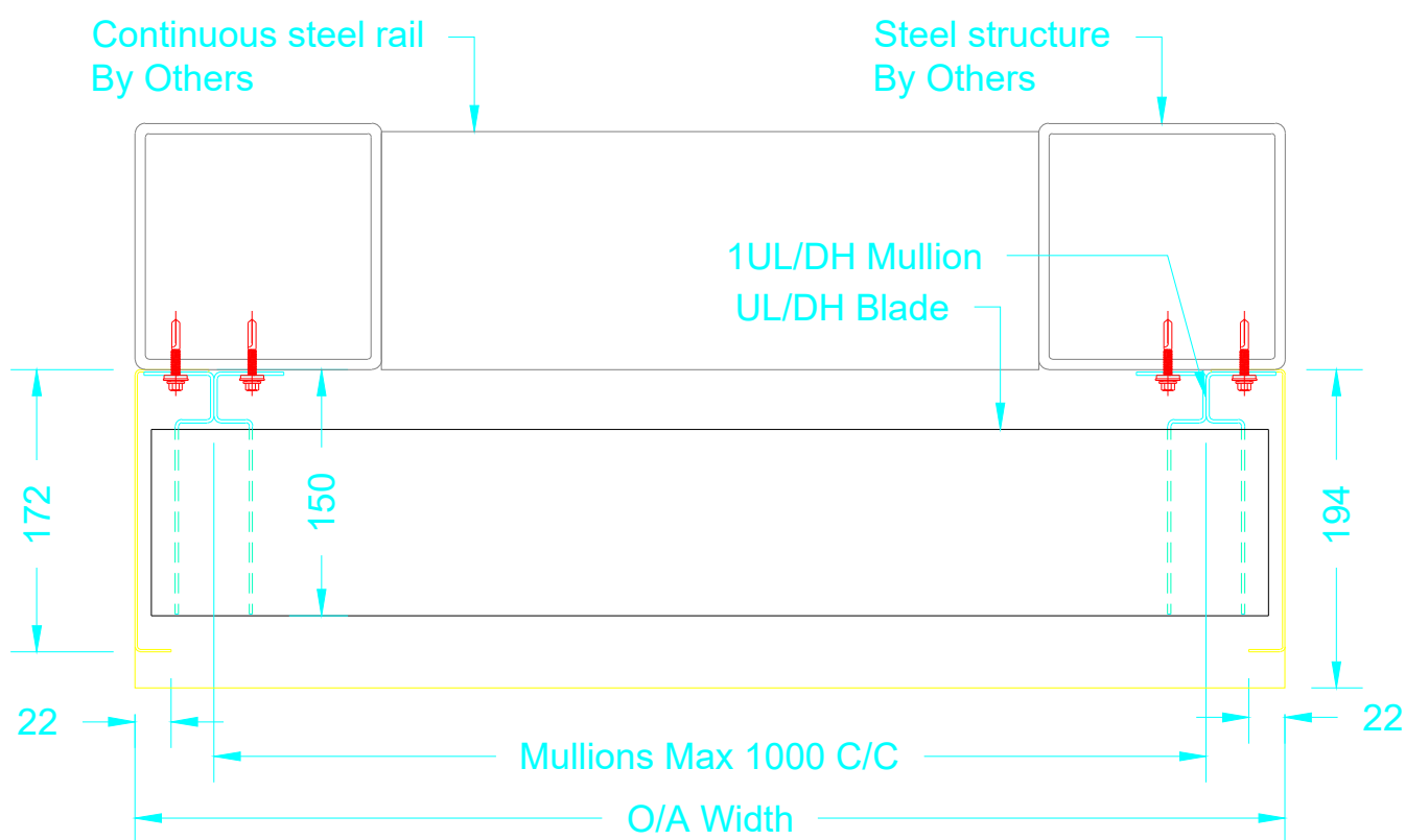
Typical 1ULDH Plan
