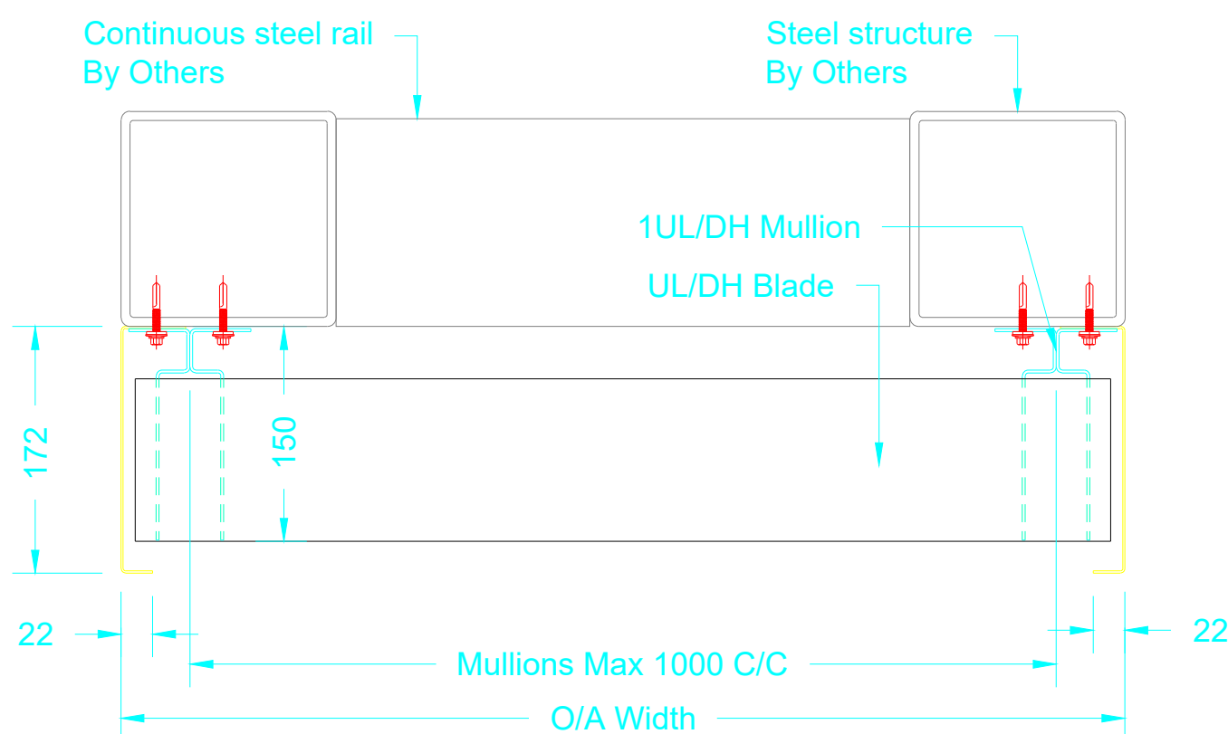
Typical 1ULDH Inverted Plan
