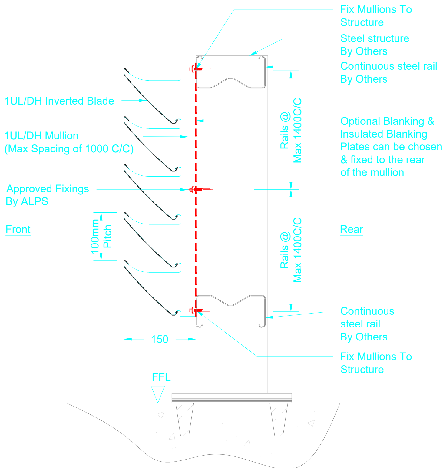
Typical 1ULDH Inverted Section
