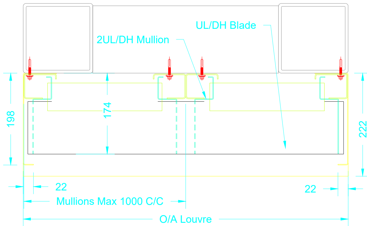
Typical 2ULDH Plan
