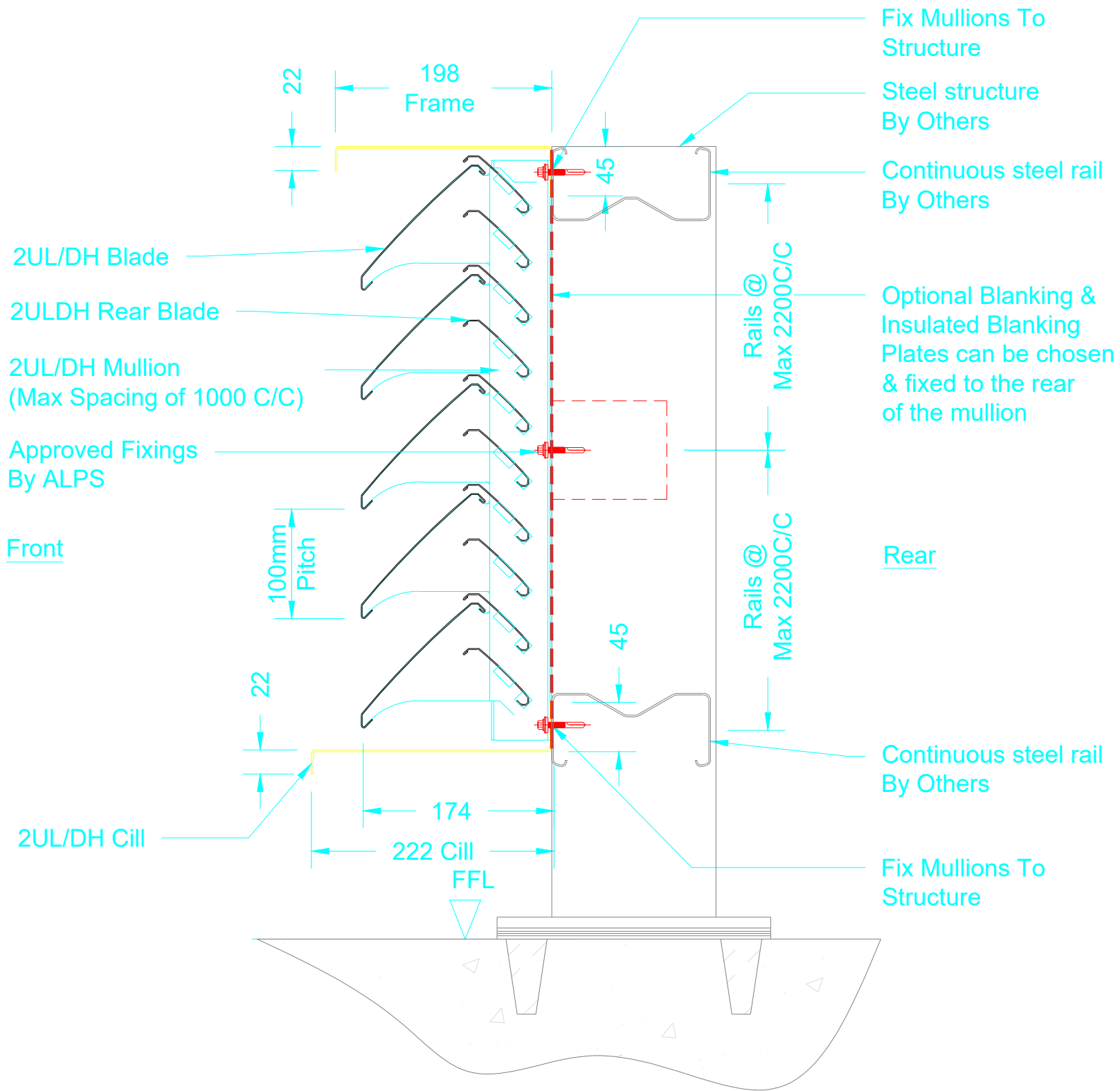
Typical 2ULDH Section
