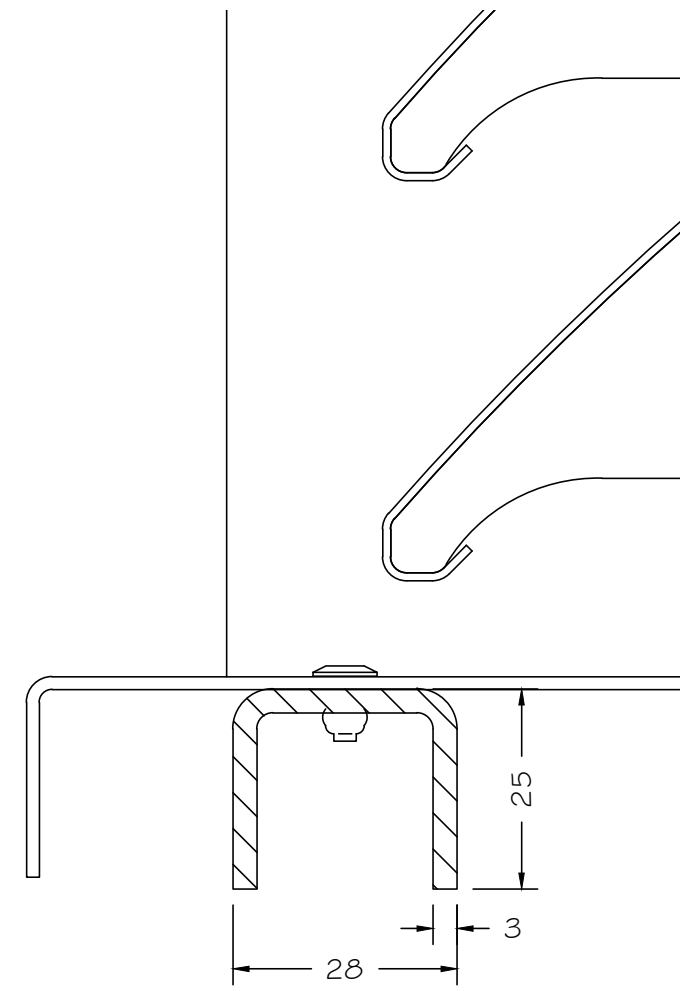
Cill detail
