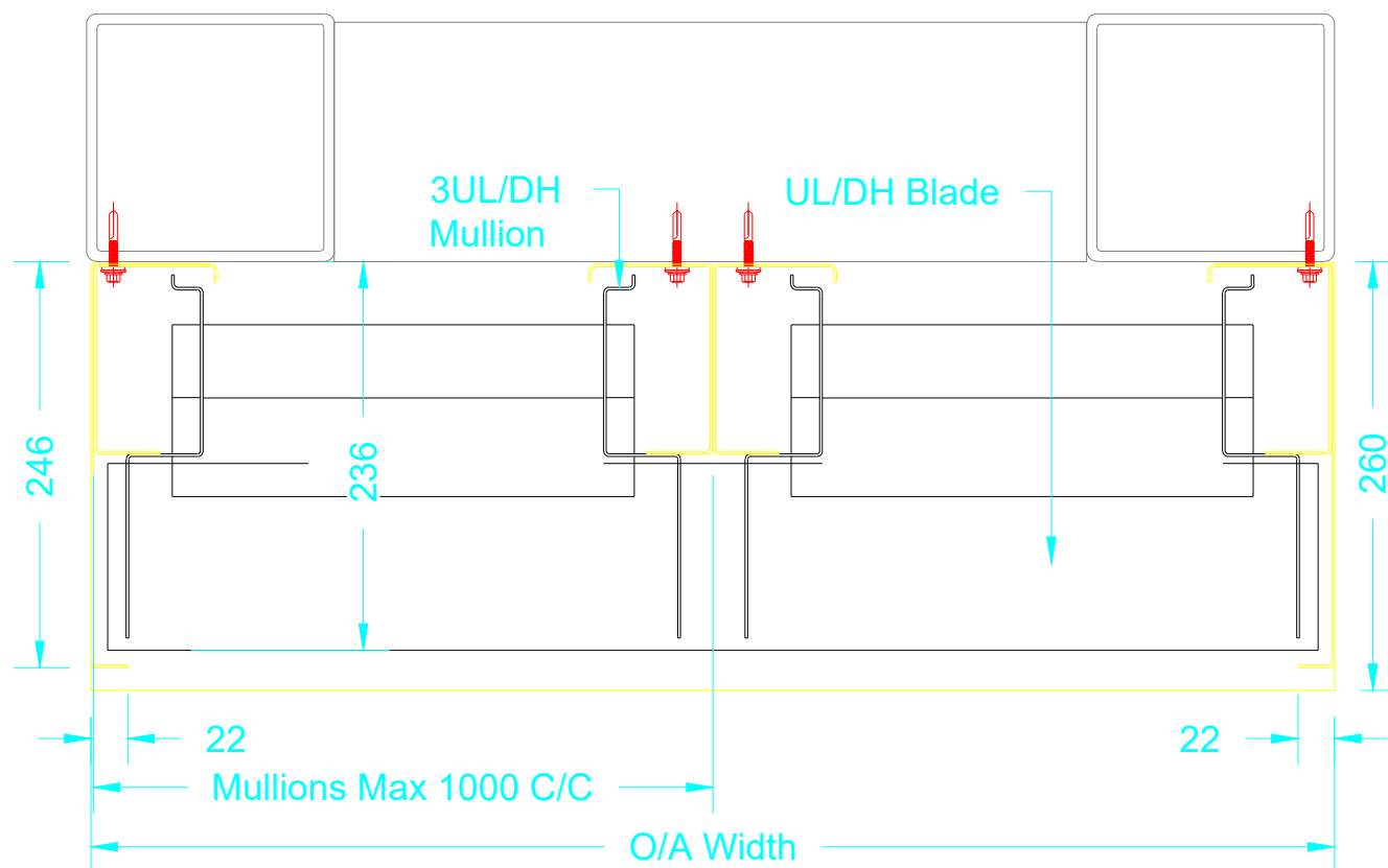
Typical 3ULDH Plan
