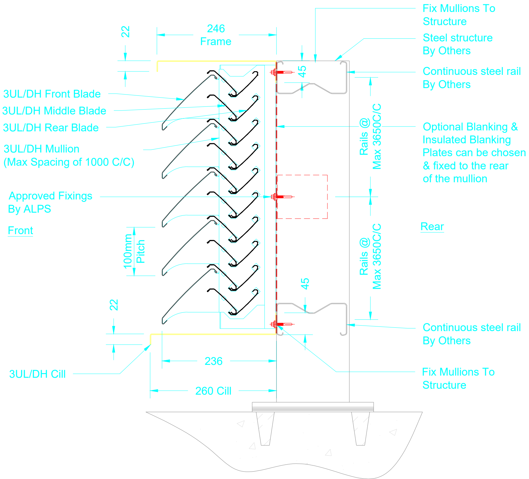
Typical 3ULDH Section
