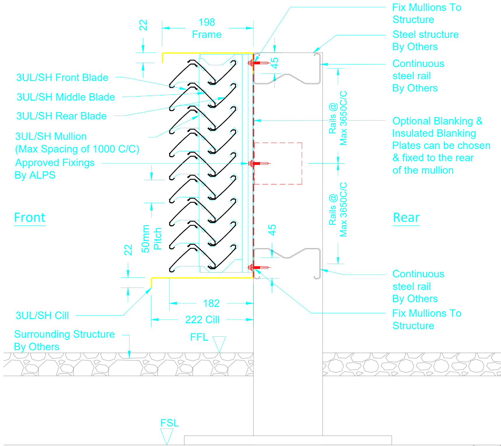
Typical 3ULSH Section
