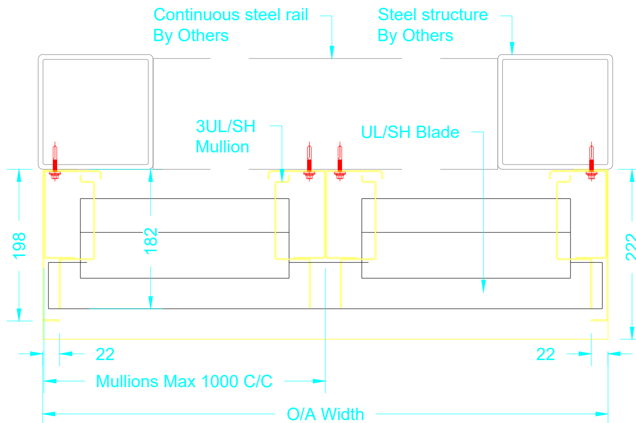
Typical 3ULSH Plan
