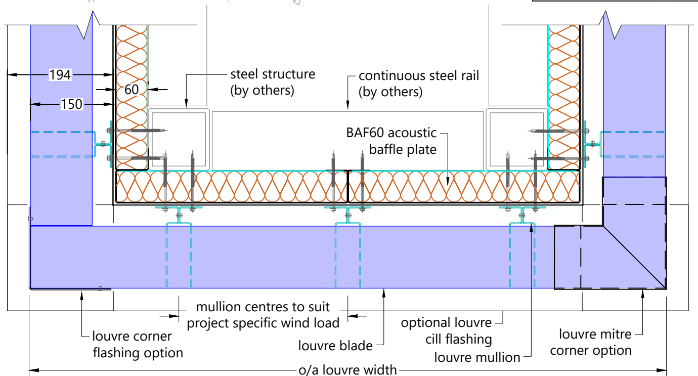
Typical 1UL/DH + BAF60 Plan
