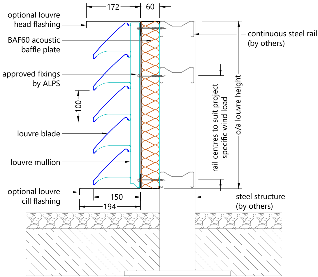
Typical 1UL/DH + BAF60 Section
