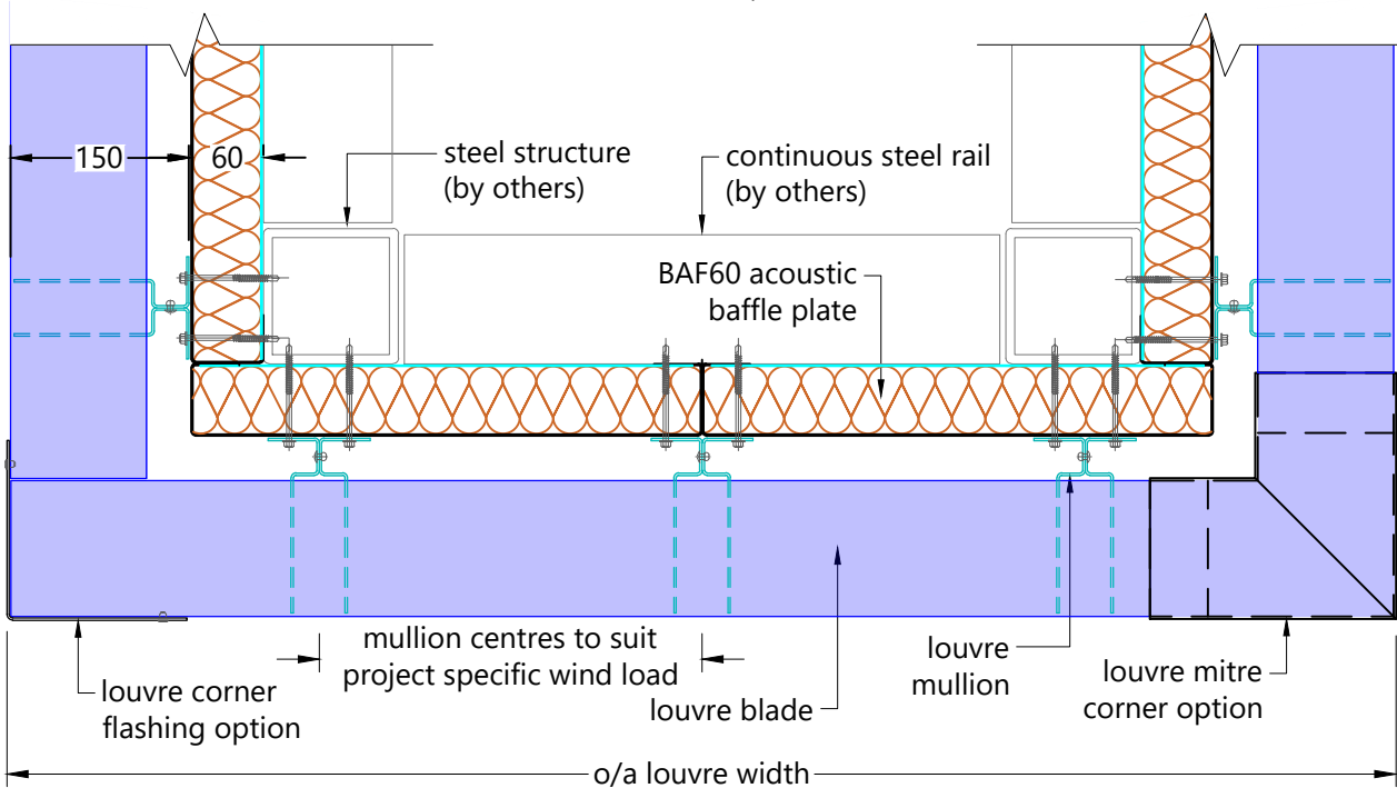
Typical 1UL/Di + BAF60 Plan
