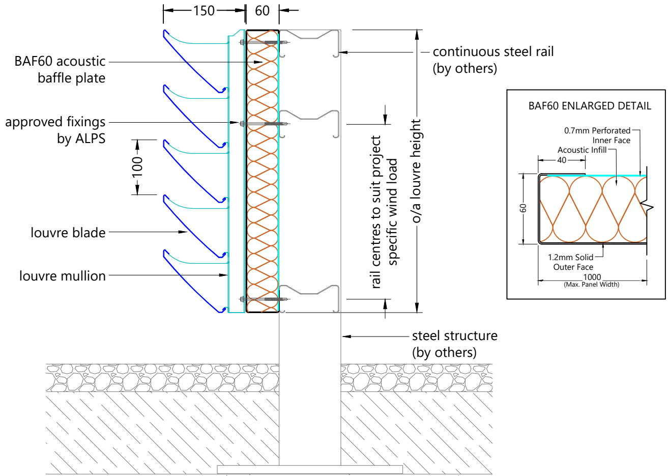
Typical 1UL/Di + BAF60 Section
