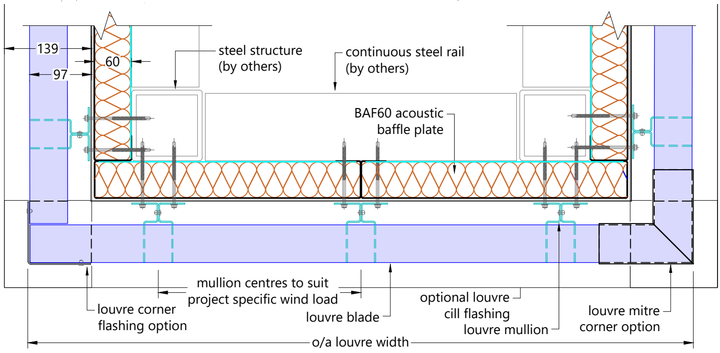
Typical 1UL/SH + BAF60 Plan
