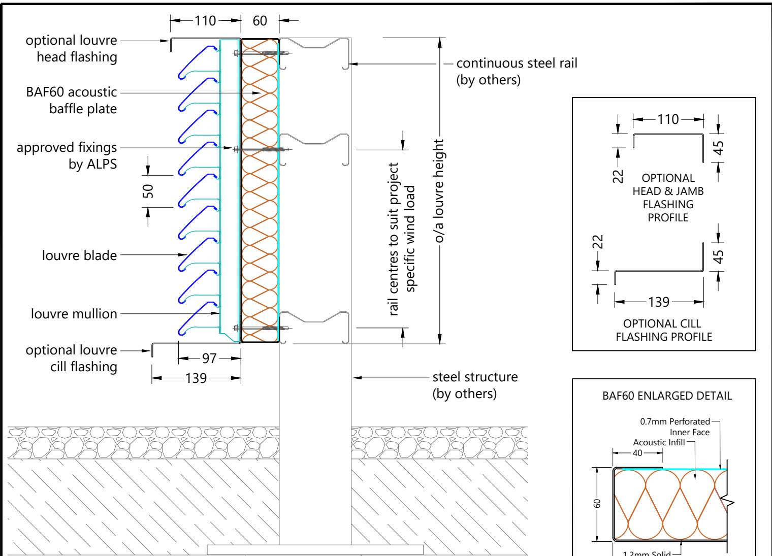
Typical 1UL/SH + BAF60 Section
