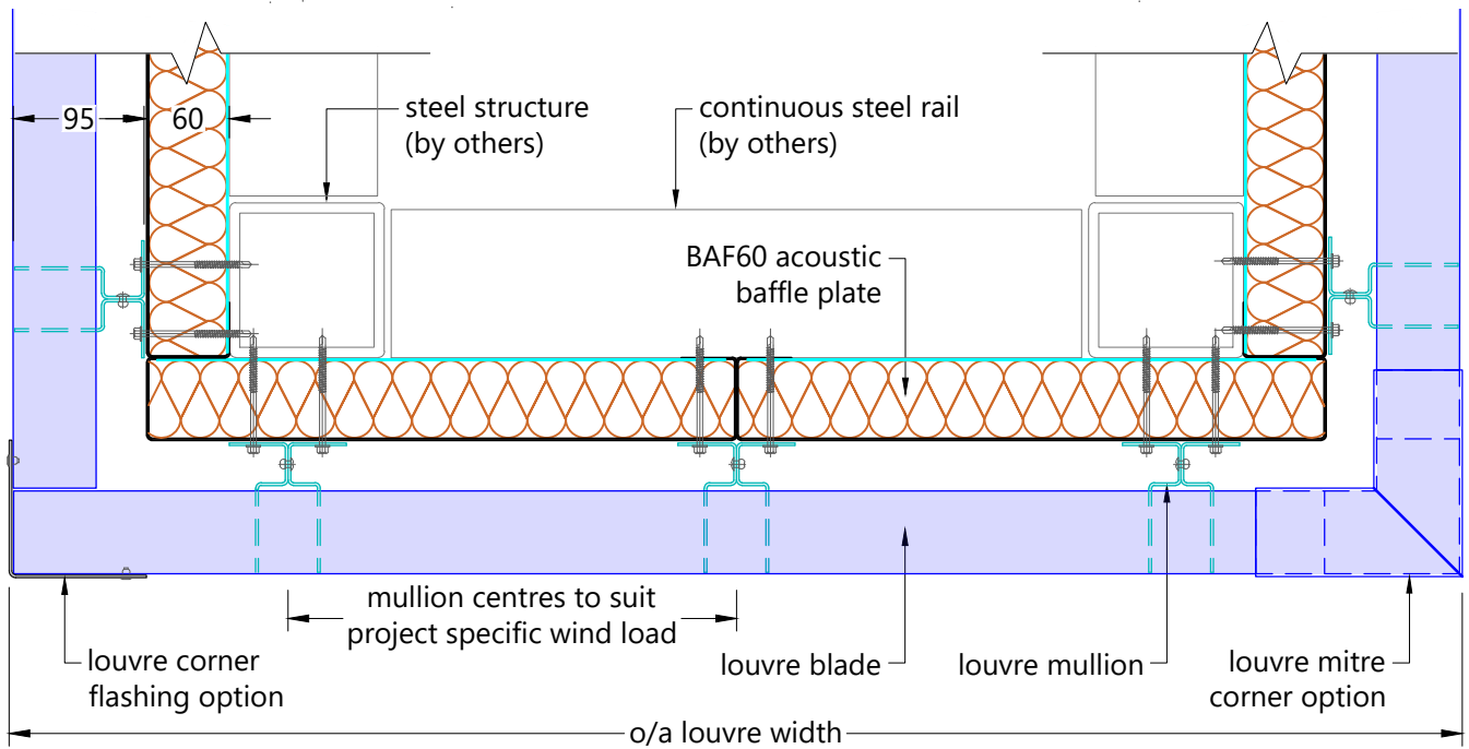
Typical 1UL/Si + BAF60 Plan
