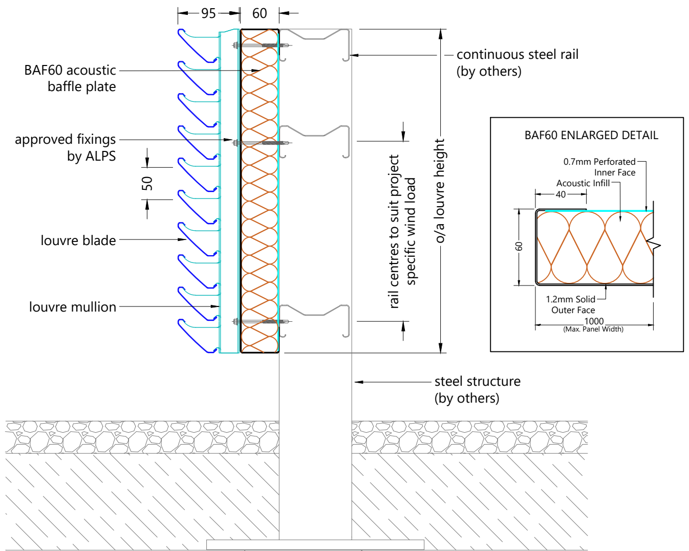
Typical 1UL/Si + BAF60 Section
